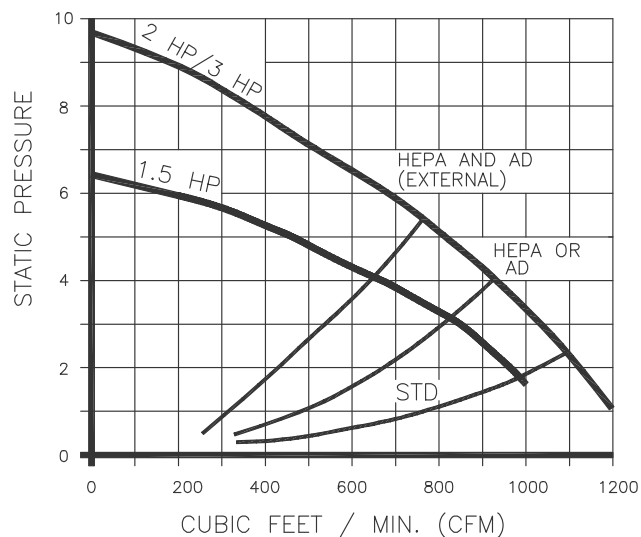
PERFORMANCE CURVES
