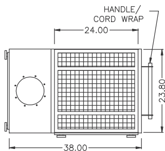
TOP VIEW (WITH OPT. HEPA/AD OUTLET SHOWN)
