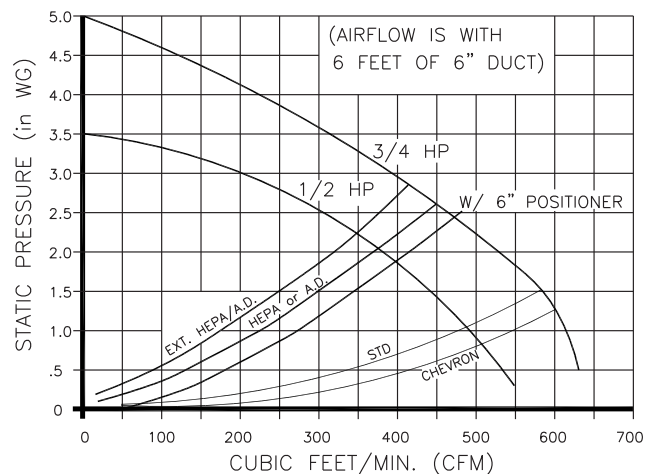
PERFORMANCE CURVES
