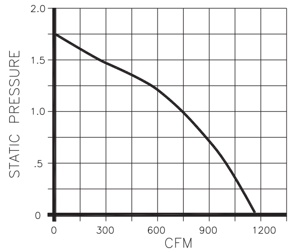
PERFORMANCE CURVES
