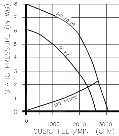
PERFORMANCE CURVES
