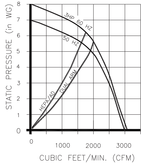
PERFORMANCE CURVES
