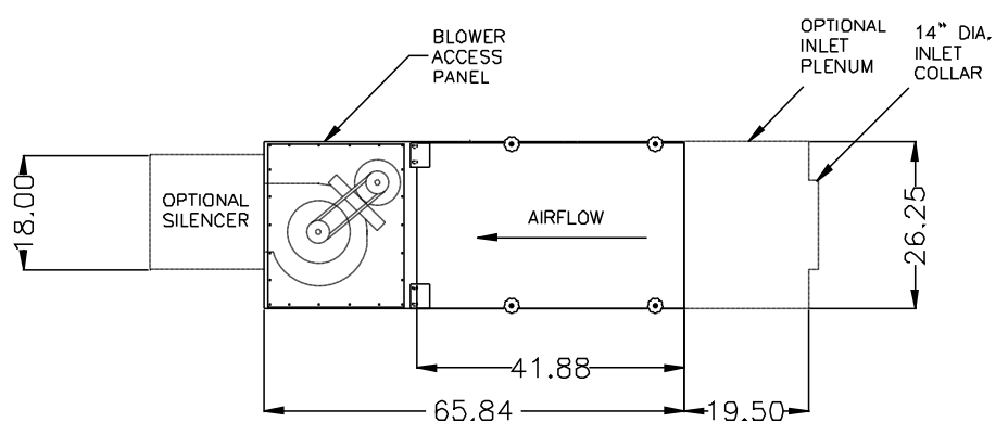
SIDE VIEW
