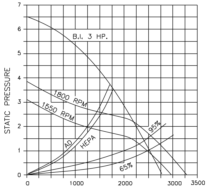
PERFORMANCE CURVES
