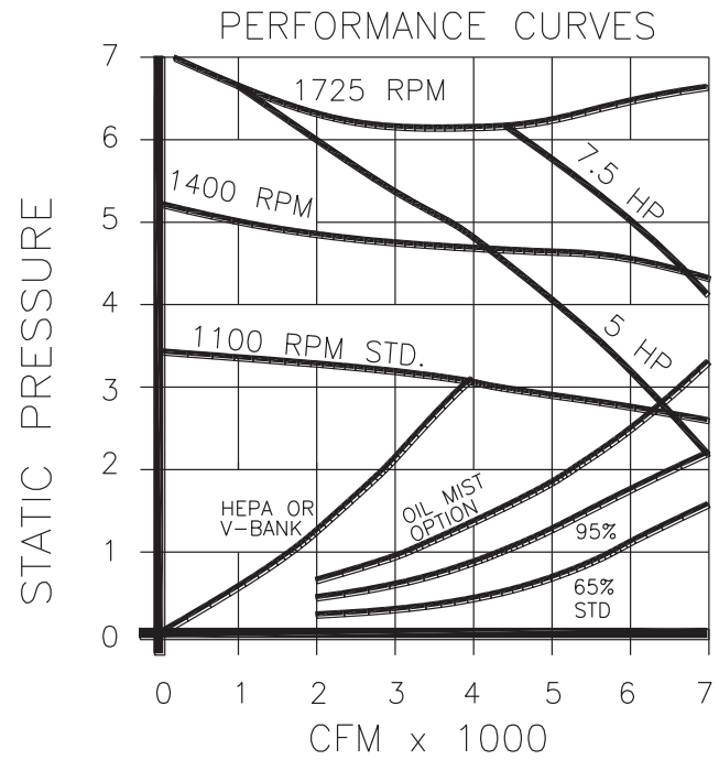
PERFORMANCE CURVES
